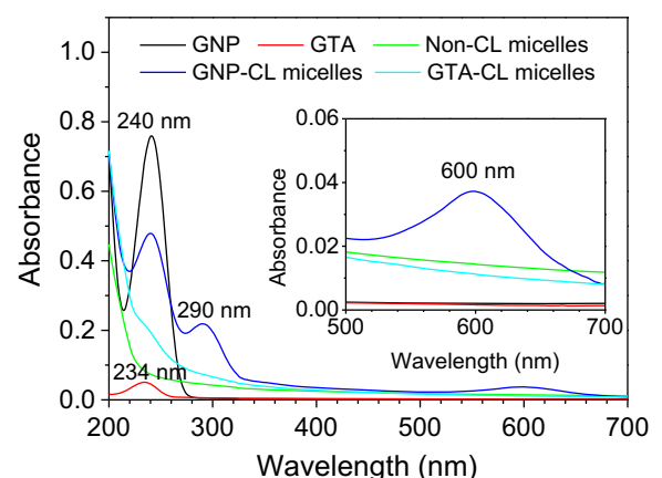
Fig. 3 UV-Vis spectra of genipin (GNP), glutaraldehyde (GTA), non-crosslinked micelles (non-CL micelles), genipin-inducing interlayer-crosslinked micelles (GNP-CL micelles), and glutaraldehyde-inducing interlayer-crosslinked micelles (GTA-CL micelles) in a scanning range of 200–700 nm
